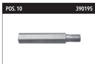
POS. 10 390195 KBZ 770 core bit extension ALU, 200 mm 11/4"
