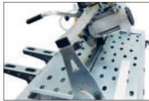
45 degree cuts from the right-hand side. The optional side table can easily be fixed on the left and right without tools.
