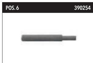
POS. 6 390254 Setting tool for impact anchor for KBZ 620 (Pos. 5) M12
