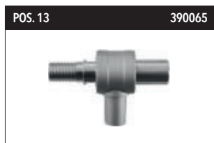
POS. 13 390065 KBZ 500 Dust extraction rotor for dry drilling Precision all-metal construction for effective dust extraction during dry drilling. increases cutting speed and the service life of the core bit, prevents "jams". Suitable for all 1 1/4" core bits. Can be used with all commercially available industrial vacuum cleaners.
